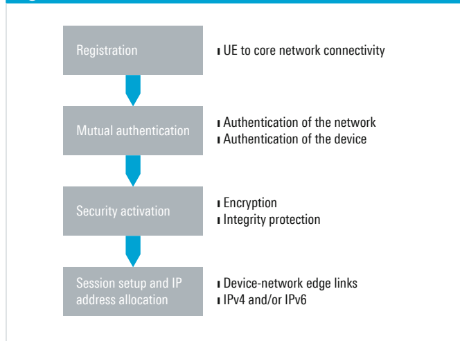
Fig. 19: Device core network interactions
