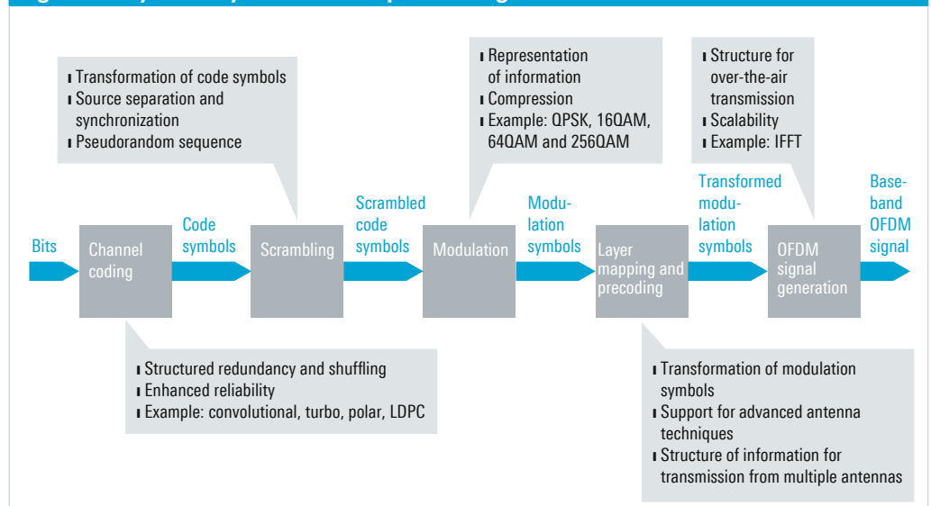
Fig. 11: Physical layer baseband processing in an OFDMA transmitter
