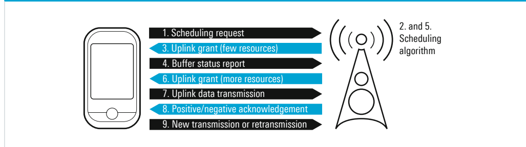
Fig. 21: Uplink data transfer steps
