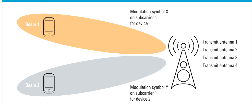
Fig. 14: Multi-user multiple input multiple output (MU-MIMO): spatial multiplexing in LTE
