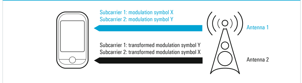
Fig. 12: Space frequency block coding: transmit diversity in LTE
