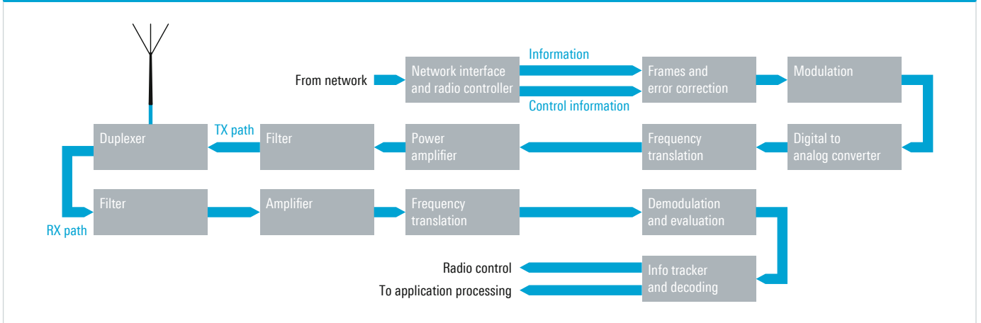
Fig. 6: Composition of an FDD system
