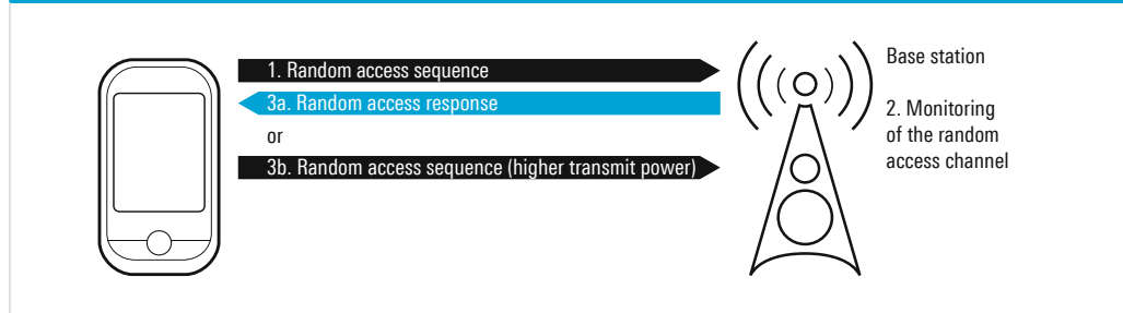
Fig. 18: An overview of the random access procedure
