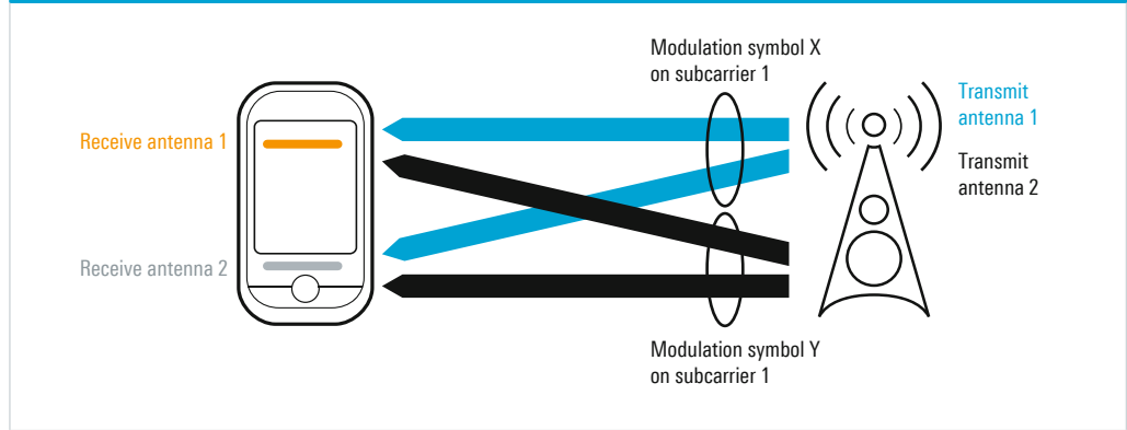
Fig. 13: Single-user multiple input multiple output (SU-MIMO): spatial multiplexing in LTE
