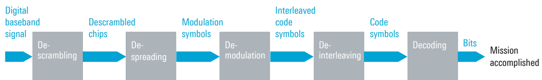
Fig. 10: Physical layer baseband processing in a CDMA receiver
