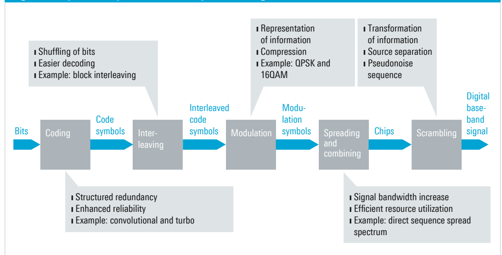
Fig. 9: Physical layer baseband processing in a CDMA transmitter
