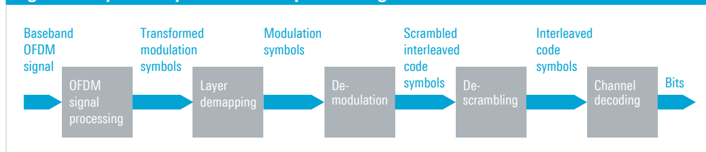
Fig. 15: Physical layer baseband processing in an OFDMA receiver
