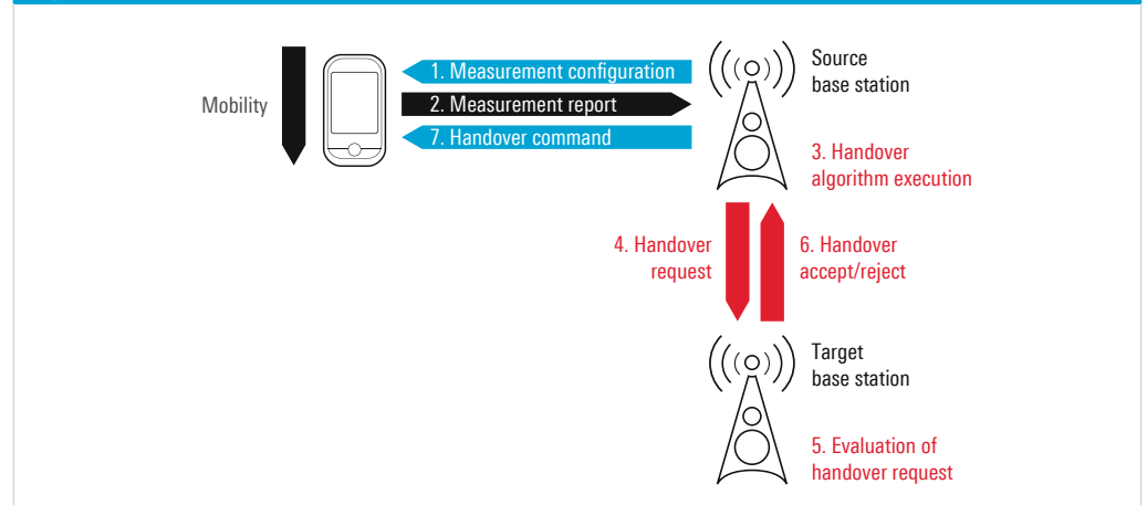
Fig. 22: Overview of handover steps
