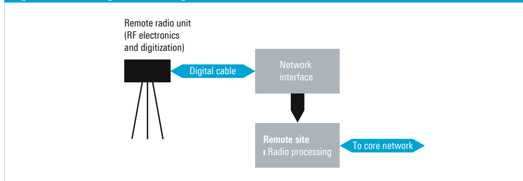
Fig. 8: BS configuration: digital cable between the RF unit and baseband unit
