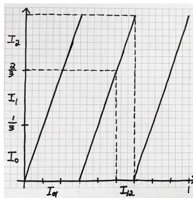
Figure 4: T_3 I_{12} = I_2 .
